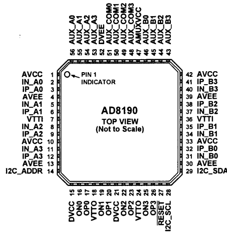
Figure 3. Pin Configuration
